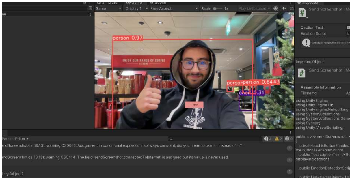
Figure 2.5.3 Object Detection
